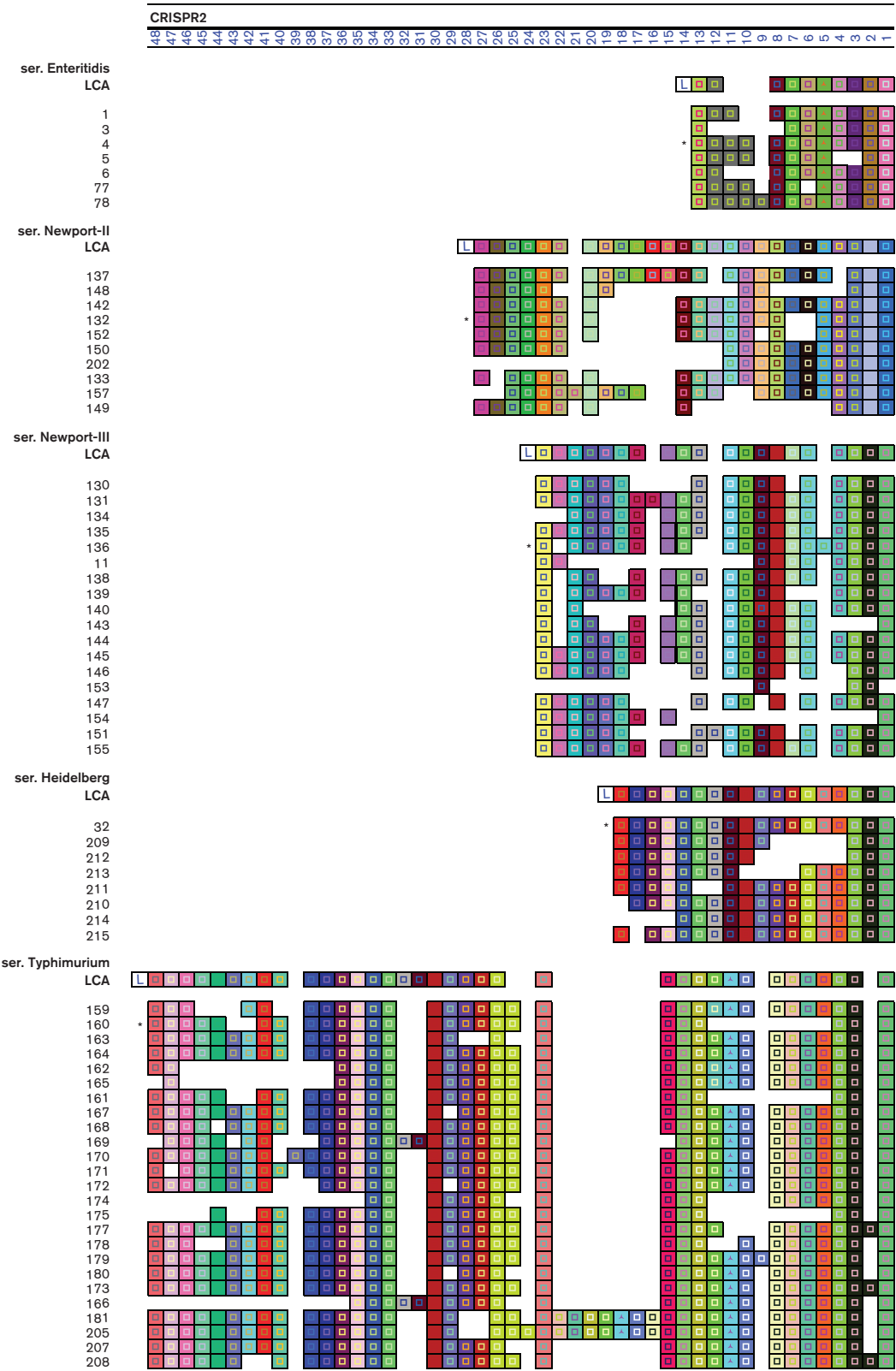
Fig. 3. Spacer organization in CRISPR2. The data are presented as in Fig. 2. In some ser. Newport-III isolates, sp15 is missing the upstream direct repeat, as indicated by a bold line. SNPs in ser. Newport-III (sp9) and Typhimurium (sp12) are shown by variations in colour of the box.
